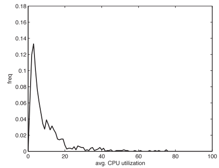
Fig. 14. Distribution of the average CPU utilization of the VMs.
