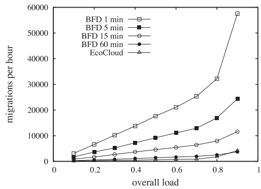
Fig. 18. Number of migrations per hour in the data center versus load: comparison between ecoCloud and BFD.
