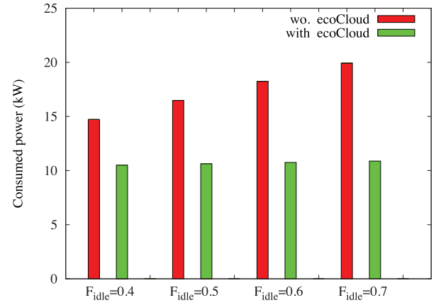
Fig. 8. Consumed power with different values of F_{idle} , before and after applying ecoCloud .
