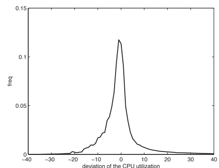
Fig. 15. Distribution of the deviation between the punctual CPU utilization and the average CPU utilization of the same VM.
